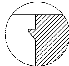
DETAIL "A" (SCALE : 3/1)
